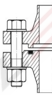
Form TG tongue and groove
