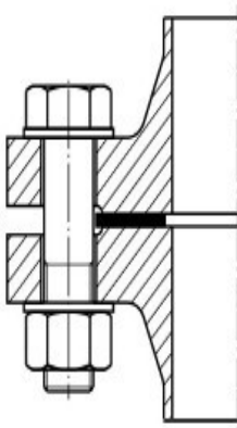
Form IBC flat face and raised face
