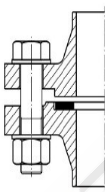
Form SR male-female
